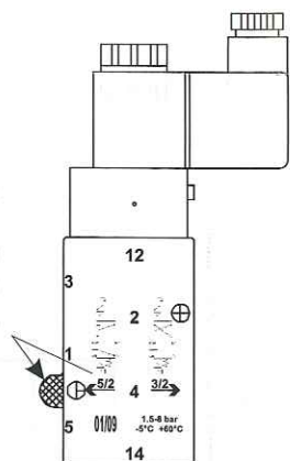
Front side showing 5/2 indication
